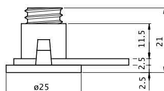
Registro Nylon vite 25mm
